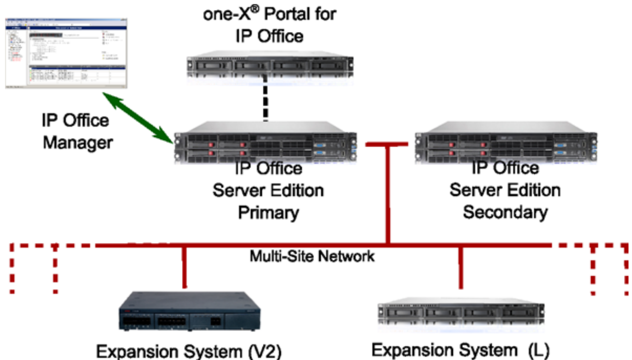
Illustration 1 : topologie de IP Office Server Edition
